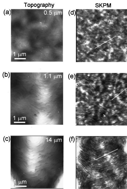
FIG. 1. AFM topographs and surface potential images of GaN films 0.5, 1.1, and 14 \mu\text{m} in thickness. The gray scales correspond to a range of 15 nm for the AFM topographs (a)–(c) and a range of 0.2 V for the surface potential images (d)–(f).
